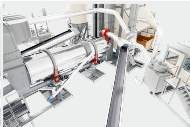
Blue smokes are filtered and cleaned and the resulting air is reused in the drying-heating process
